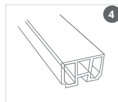
100 x 66 x 1480mm Top+Bottom Rail
